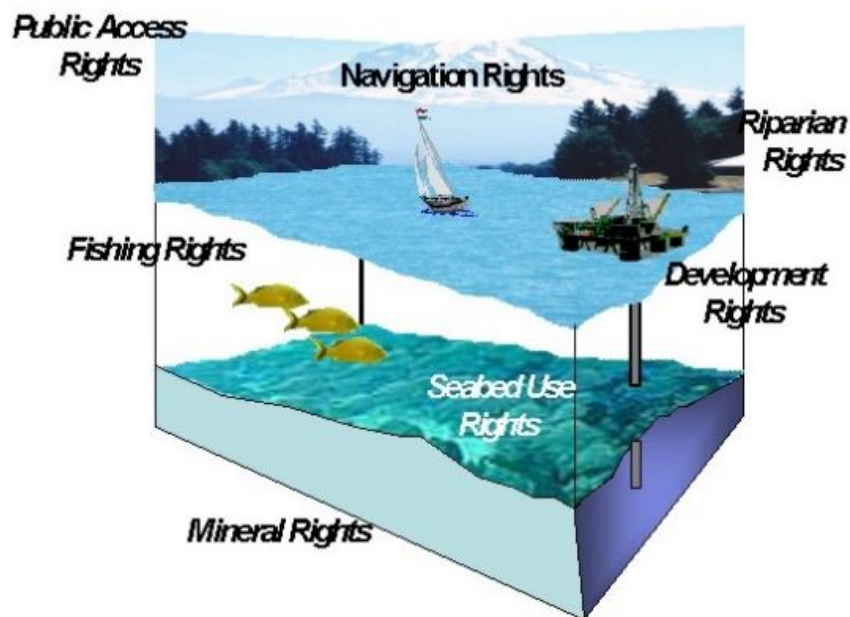
Figure 1: The Marine Parcel (after Sutherland, 2001)
